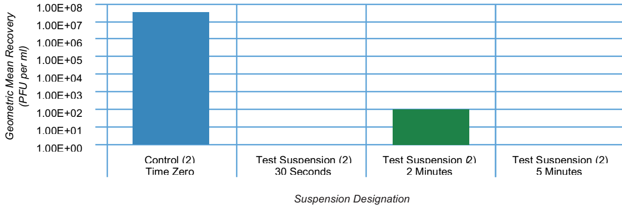
Figure 3. Modified ASTM E1052 Test: MS-2 Bacteriophage Data
