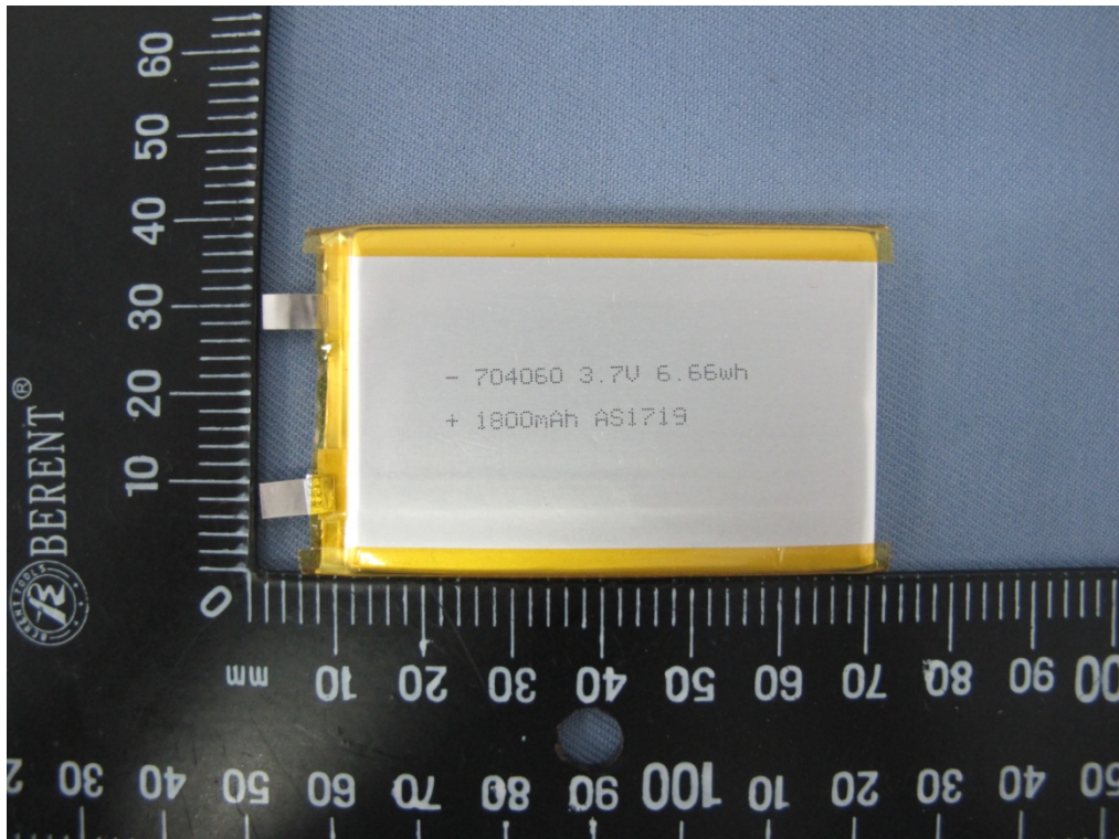
Figure 3 Internal view of battery (内部结构图)
